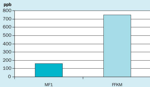
Result of a leach out test in UPDI, 85°C/1 week / 185°F/1 week according to SEMI Standard F57-0301 (20 cations)
