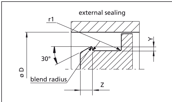
Figure 8 Groove design
