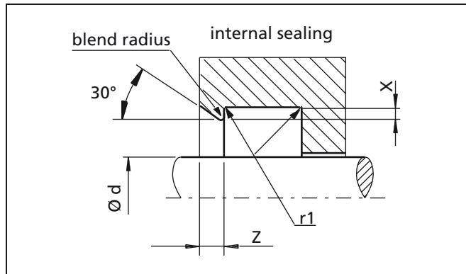
Figure 9 Groove design
