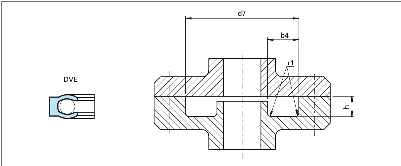
Figure 20 Installation drawing
