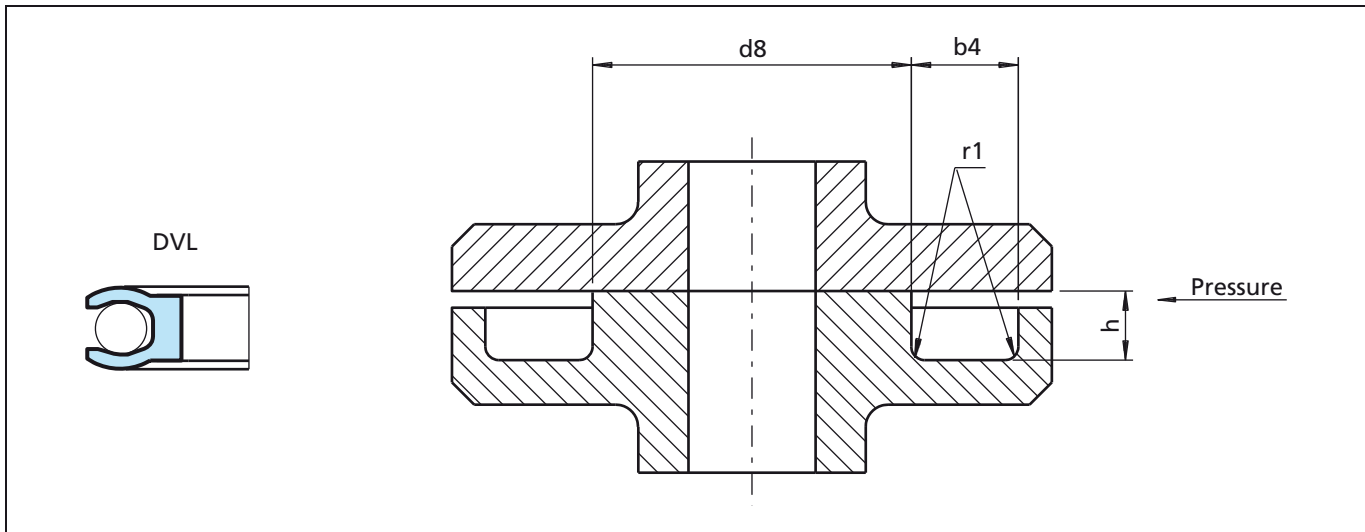
Figure 21 Installation drawing
